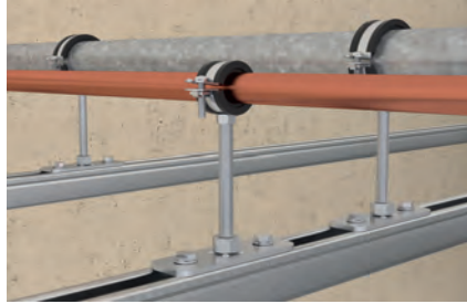
Baseplate on installation channel
